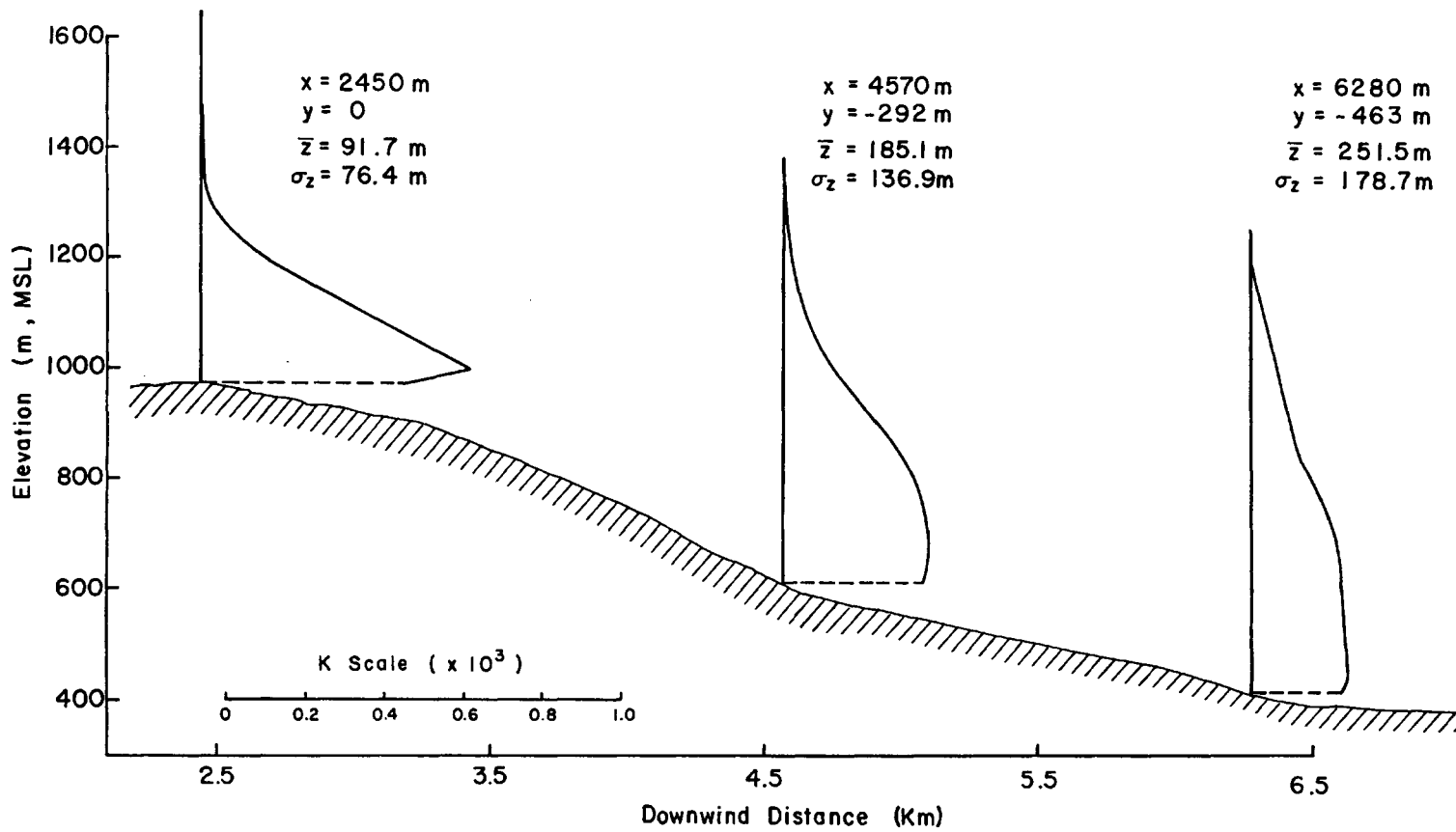
Figure 5-6. Vertical Concentration Distribution Downwind of Unit 20A for u_\infty = 20 \text{ m/s} .
