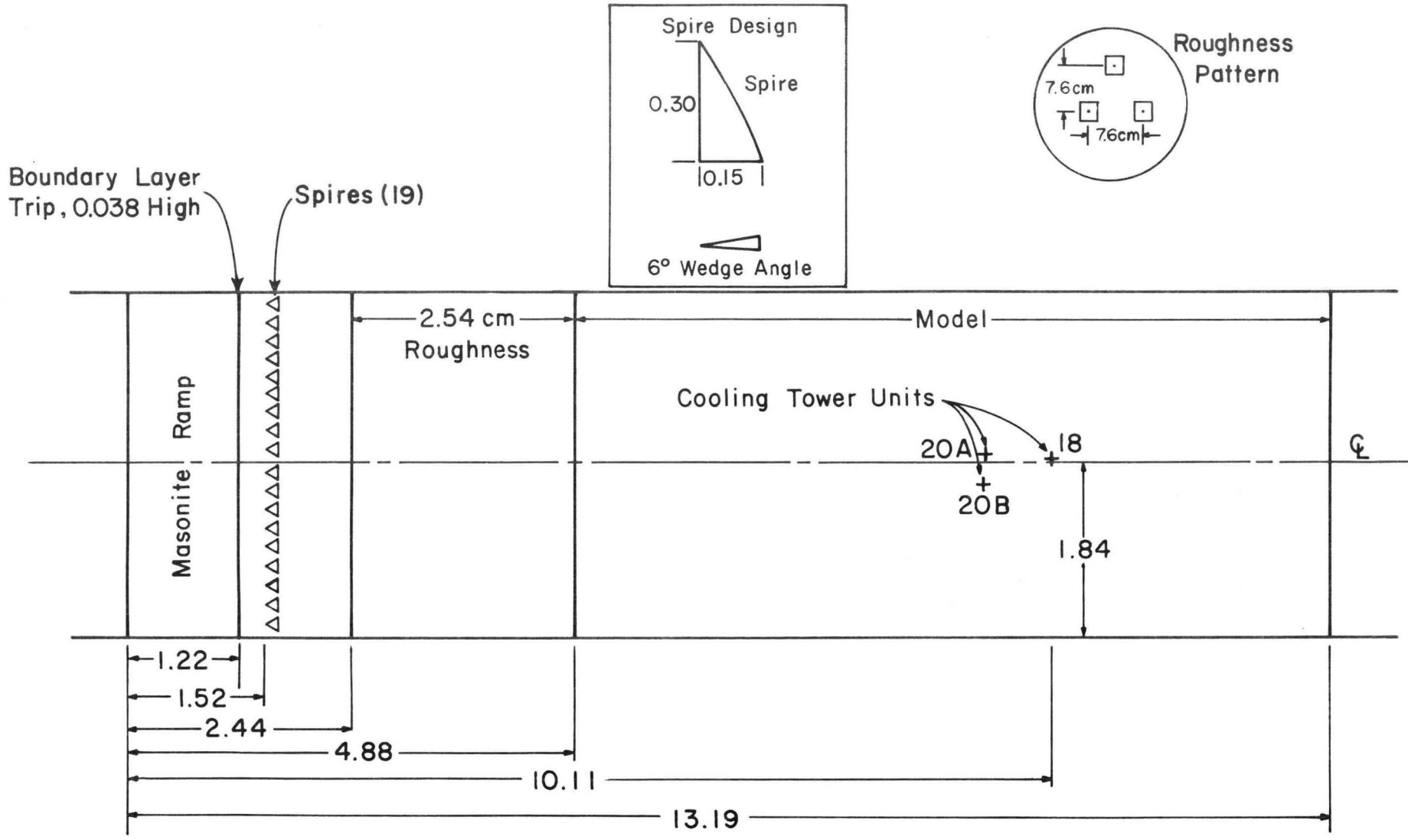
Figure 3-6. Wind Tunnel Set-up for Neutral Stability Tests
